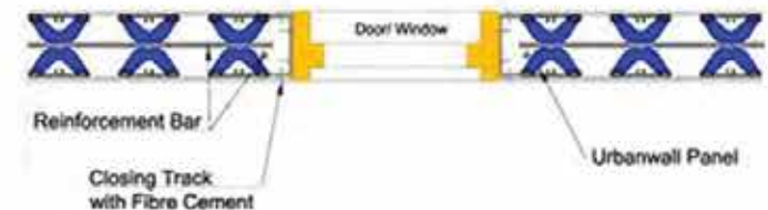
TYPICAL OPENING DETAIL (100mm panel)
